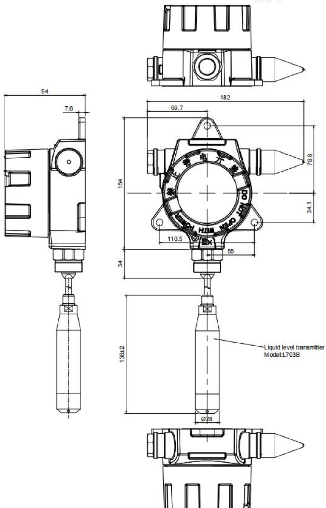
Level Sensor, model No. MZW2603
