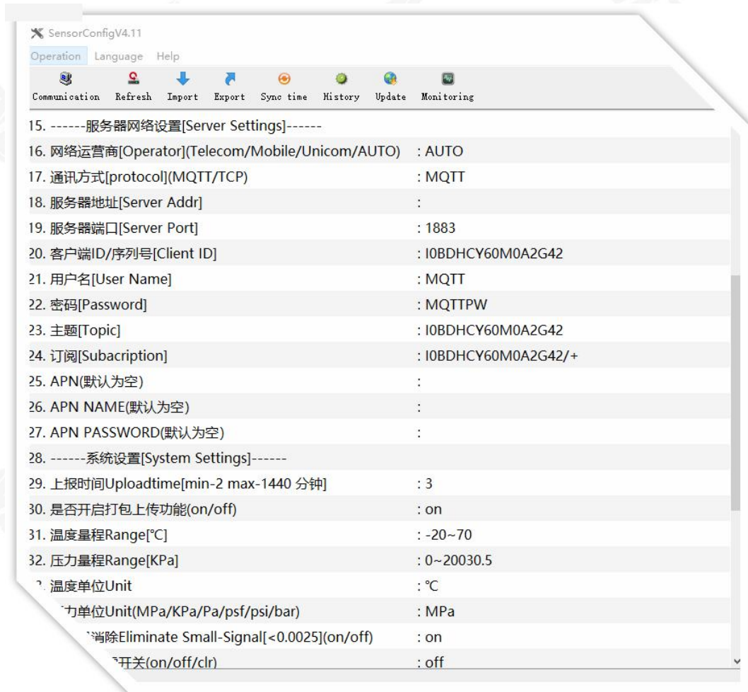
Third Party Server IP address / Server Port / APN Setting
